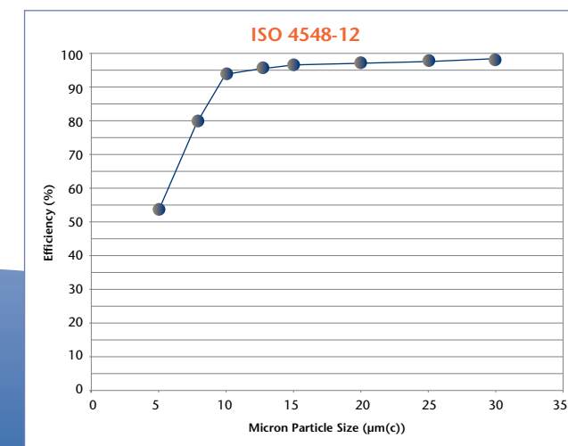
Particle Removal Efficiency vs. Particle Size.
