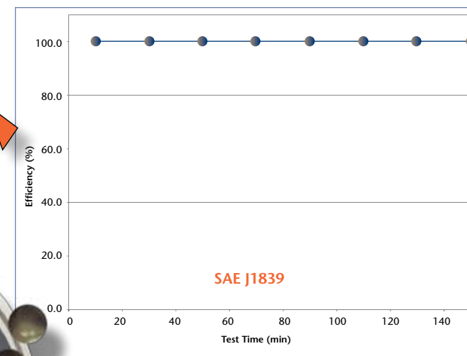
Sierra's 10 Micron Fuel Water Separating Filter Performance Test Over 99% Separation of Emulsified Water
